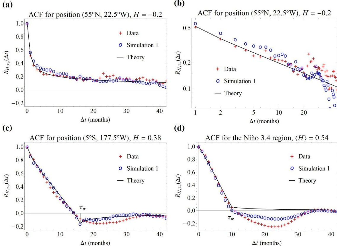
Figure S8. Autocorrelation functions (ACF's) for the reference dataset (marked as “+”), for one set of simulations (marked as “o”) and obtained theoretically using Eqs. (S3) or (S4) (solid curve) for the temperature series at different positions: (a) grid point in the North Atlantic at (55°N, 22.5°W), with estimated H = -0.2 ; (b) same as in (a) but with logarithmic scale in both axes to highlight the scaling; (c) grid point in the Tropical Pacific at (5°S, 177.5°W), with H = 0.38 and \tau_w = 16 months and (d) the monthly mean temperature for the Niño 3.4 region (5°N-5°S, 170°W-120°W), with average \langle H \rangle = 0.54 and \langle \tau_w \rangle = 10 months.
